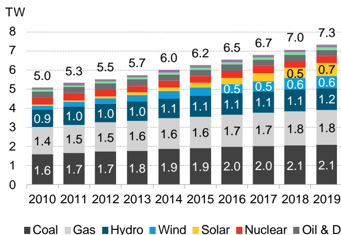
Figure 22: Global installed capacity by technology
