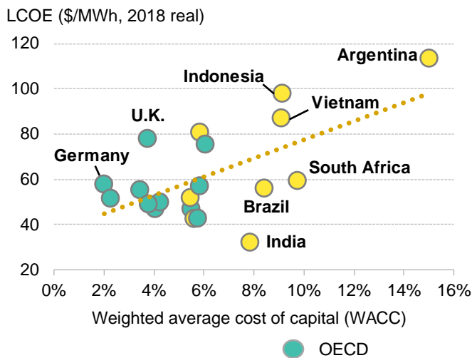
Figure 69: Financing cost impacts on levelized costs of electricity, utility-scale PV
