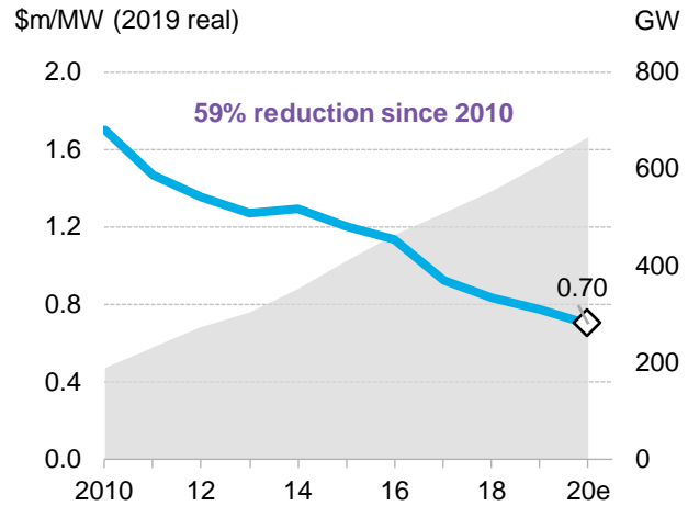
Figure 66: Benchmark onshore wind turbine price (left axis) and cumulative installed capacity (right axis)
