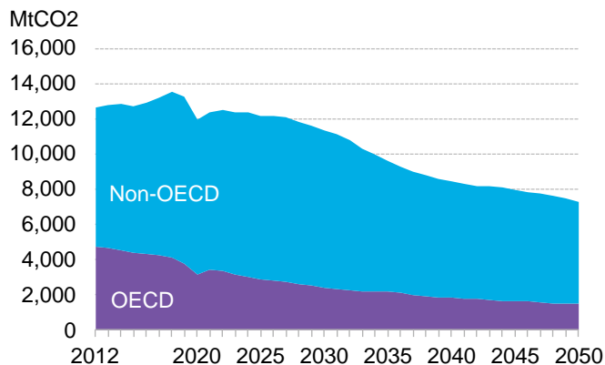
Figure 18: Projected power sector CO2 emissions
