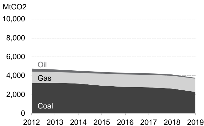
Figure 1: Developed countries' estimated power sector CO2 emissions by technology
