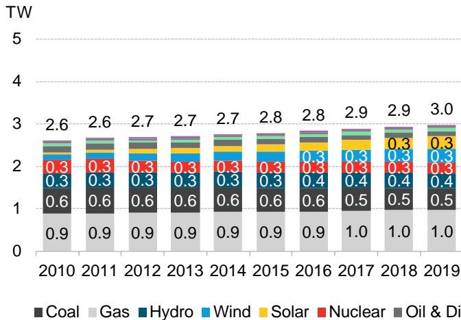
Figure 27: Cumulative capacity by technology in developed markets
