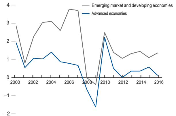
Figure 1: Total Factor Productivity 2000–2016 PPP, GDP-weighted
