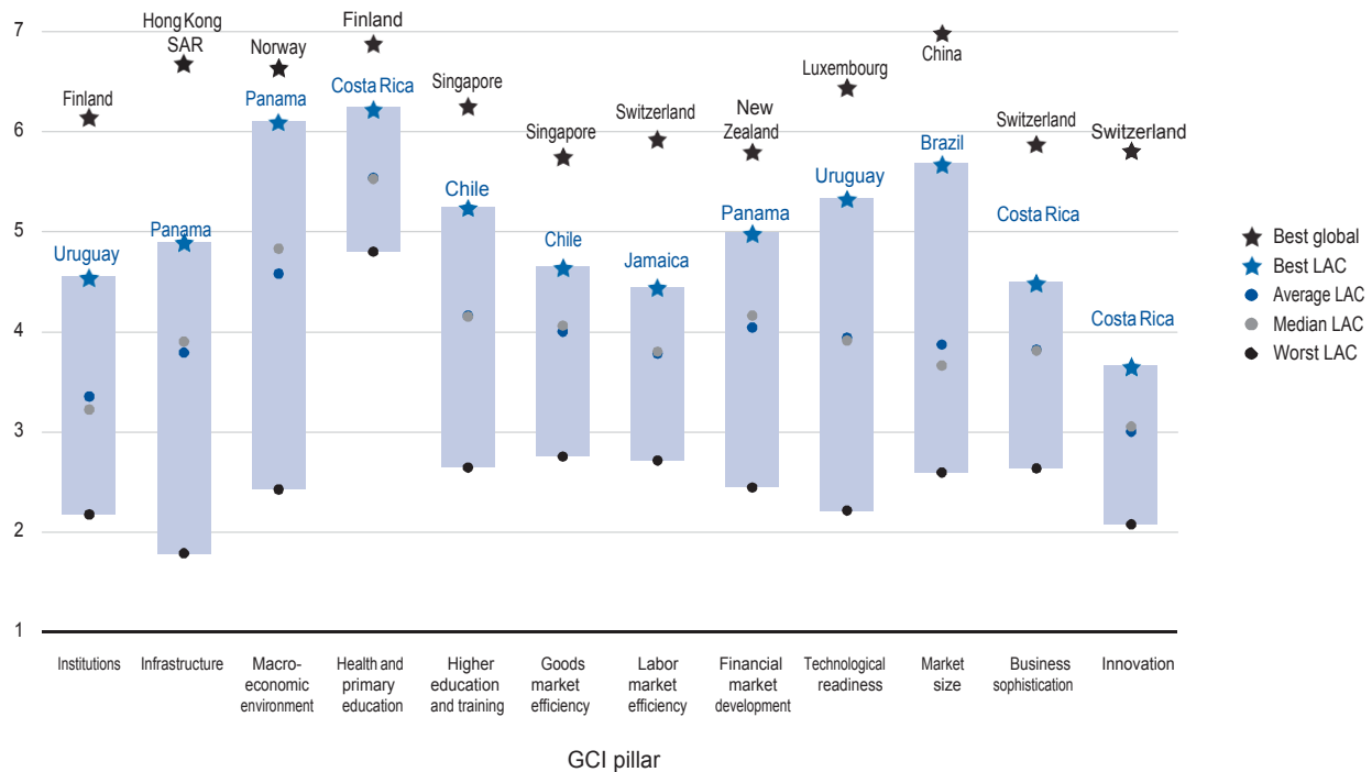
Figure 5: GCI score range for Latin America and the Caribbean (LAC) across the 12 pillars, 2017–2018 edition Score (1–7)
